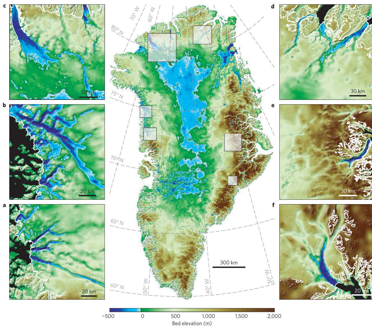
Figure 1 | Bed elevation of the Greenland ice sheet colour-coded between -500 and +2,000 m, with submarine areas in blue. Details of the large-scale map for Upernavik Isstrøm and Nunatakassaap Sermia (a), Hayes Gletscher, Allison Gletscher and Illullip Sermia (b), Petermann, Steensby and Ryder Gletscher (c), Marie Sophie Gletscher, Academy Gletscher and Hagen Bræ (d), F. Graae, Charcot and Daugaard-Jensen (e), and Kangerlussuaq Gletscher (f); glaciers are listed in clockwise order. The white contour line delineates the limit of land ice. The mass conservation method is employed for the glaciers. Kriging is used to map the interior regions.
